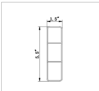
I555 Ribbed Rail Thickness: 0.08"
