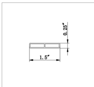
Lattice Rail
