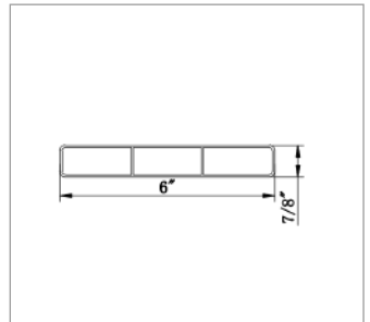
6078 Picket
