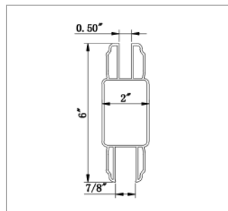
2060 Lattice Slot Rail Thickness: 0.08"
