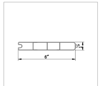
6010 T&G Thickness: 0.06"
