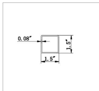
I515 Picket Thickness: 0.08"
