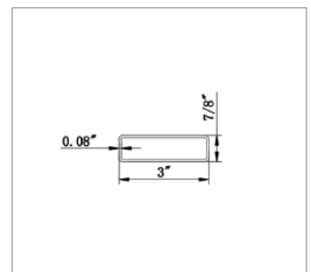
3078 Picket Thickness: 0.08"
