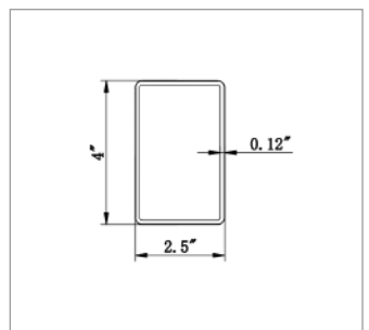
2540 Post
