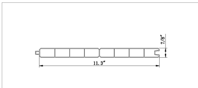
I1378 2-Section T&G Thickness: 0.055"
