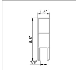
I555 Slot Rail Thickness: 0.08"
