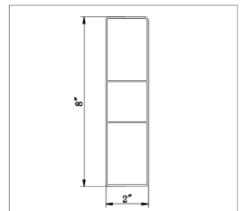
2080 Rail Thickness: 0.08"
