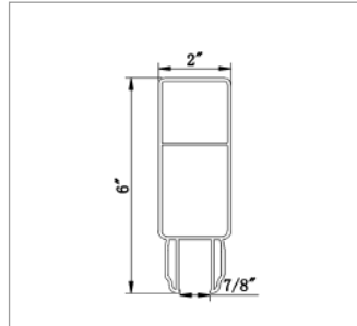
2060 Slot Rail-I Thickness: 0.09"
