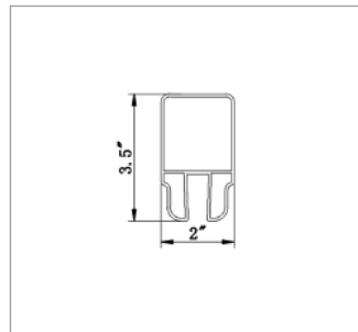
2035 Lattice Rail Thickness: 0.08"
