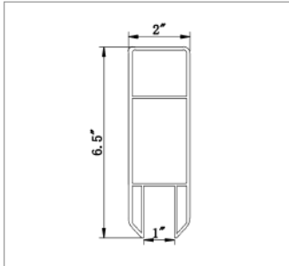
2065 Slot Rail Thickness: 0.10"
