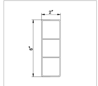
2060 Ribbed Rail Thickness: 0.087"
