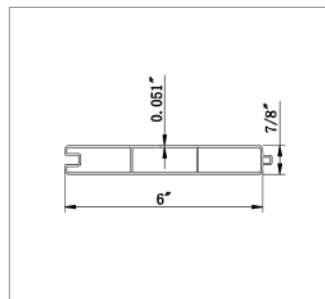
6078 T&G Thickness: 0.051"
