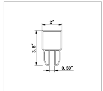
2035 Lattice Rail Thickness: 0.08"
