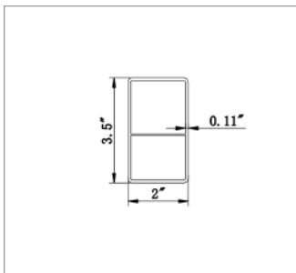
2035 Ribbed Rail Thickness: 0.11"
