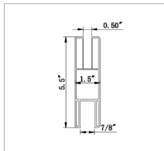
I555 Lattice Slot Rail Thickness: 0.08"
