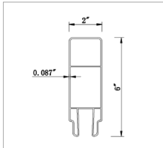
2060 Slot Rail-2 Thickness: 0.087"
