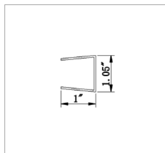
U Channel For T&G
