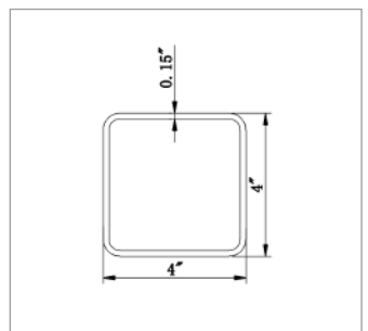
4040 Post
