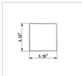
8585 Post
