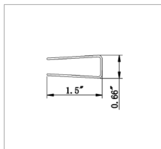
U Channel For Lattice
