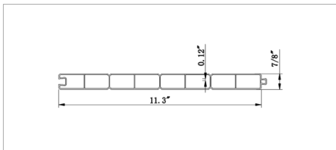
I1378 T&G Thickness: 0.051"
