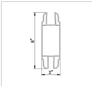
2060 Double Slot Rail Thickness: 0.08"
