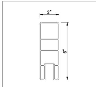
2060 Slot Rail-3 Thickness: 0.087"
