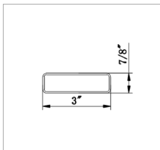
3078 Picket
