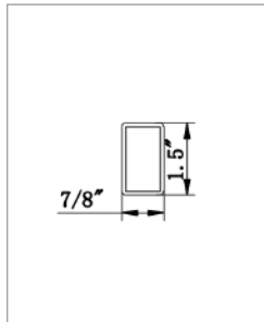
1578 Picket
