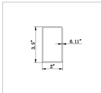
2035 Open Rail Thickness: 0.11"
