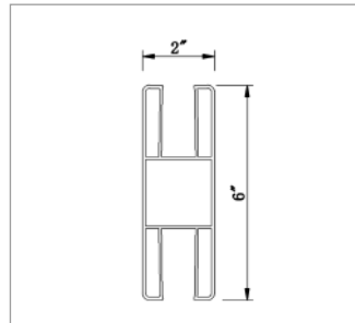
2060 Double Slot Rail For Panel Thickness: 0.08"
