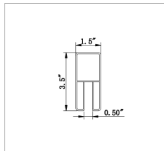
I535 Lattice Rail Thickness: 0.08"
