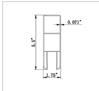
I7555 Slot Rail Thickness: 0.071"
