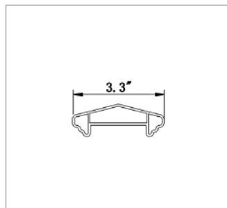
Deco Rail Thickness: 0.08"
