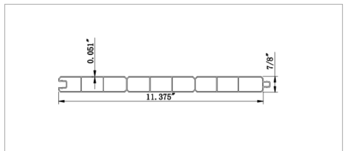
I1375 T&G Thickness: 0.051"
